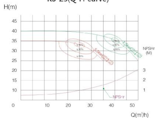
KS-25(Q-H曲线图) KS-25(Q-H curve)
