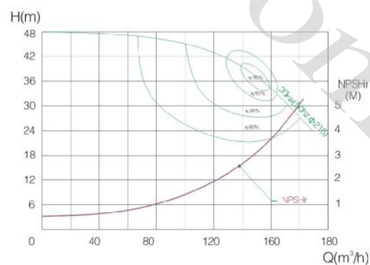
KS-50(Q-H曲线图) KS-50(Q-H curve)
