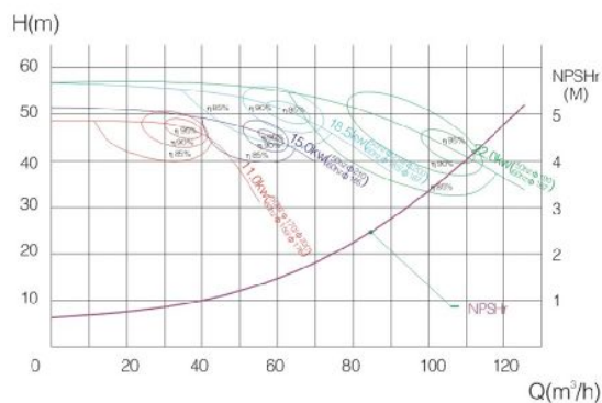
KS-40(Q-H曲线图) KS-40(Q-H curve)
