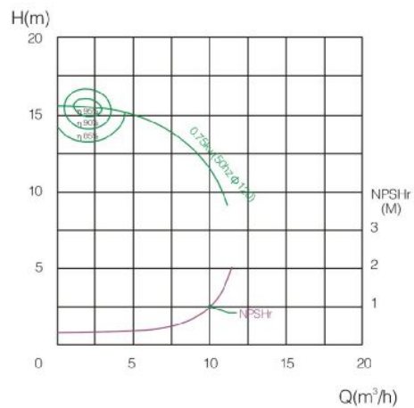
KS-5(Q-H曲线图) KS-5(Q-H curve)
