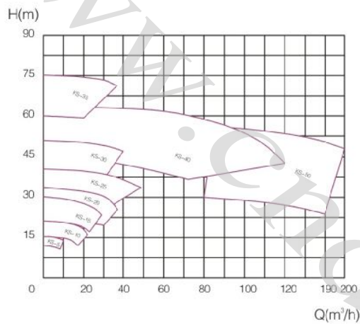
(KS)泵Q-H曲线图 KS series Q-H curve figure
