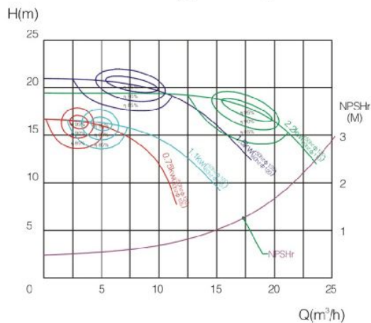
KS-10(Q-H曲线图) KS-10(Q-H curve)
