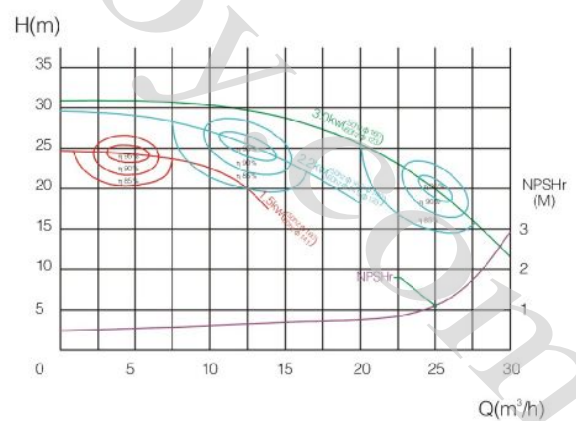
KS-15(Q-H曲线图) KS-15(Q-H curve)
